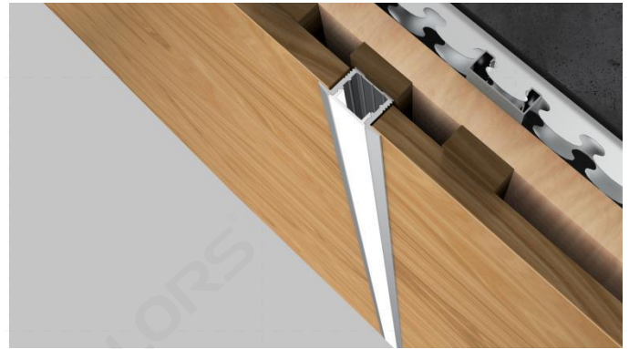
Example of application: wooden decorative board on the wall Cutout:W18*D13mm fixed by glass cement/self-tapping screws
